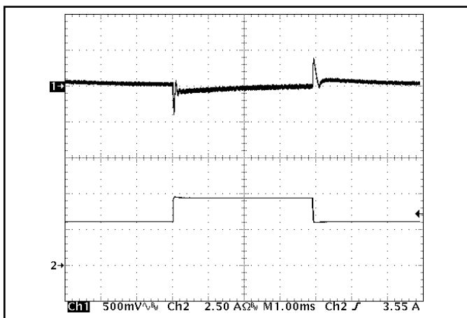
Figure 11: Output voltage response to step-change in load current (50%-75%-50% of I out (max); dl/dt = 0.1A/μs). Load cap: 10μF, 100 mΩ ESR tantalum cap and 1μF ceramic cap. Ch 1: V out (500mV/div), Ch 2: I out (2.5A/div).
