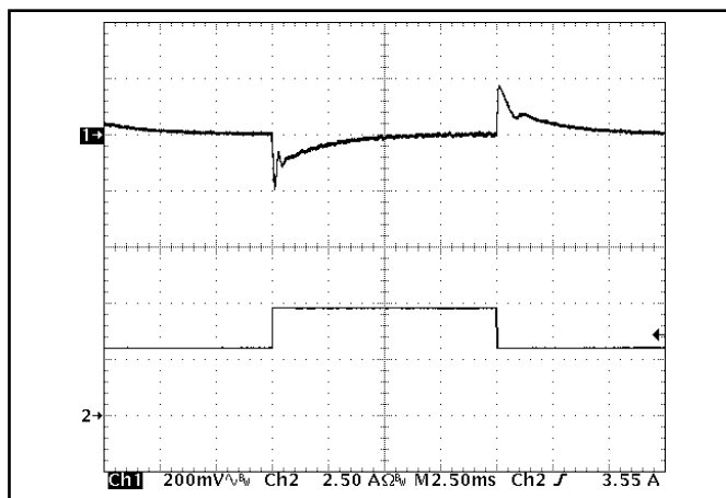
Figure 12: Output voltage response to step-change in load current (50%-75%-50% of I out (max); dl/dt = 1A/μs). Load cap: 470μF, 30 mΩ ESR tantalum cap and 1μF ceramic cap. Ch 1: V out (200mV/div), Ch 2: I out (2.5A/div).
